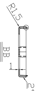
Cover
