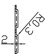
Rubber Button
