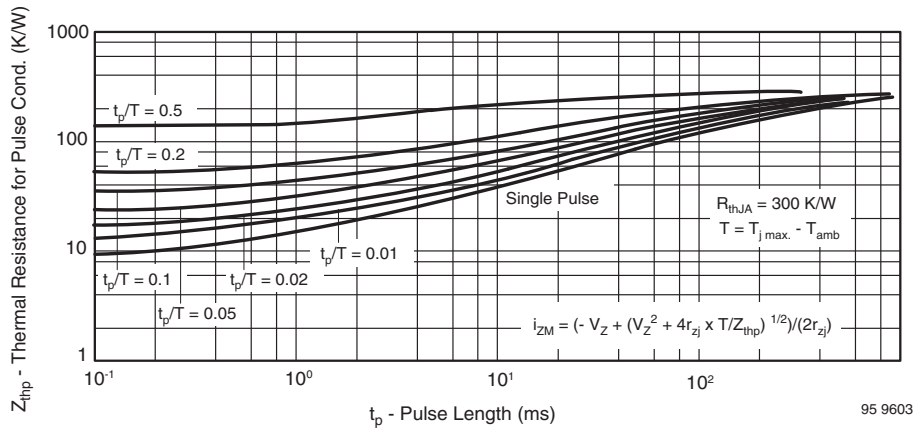
Fig. 10 - Thermal Response
