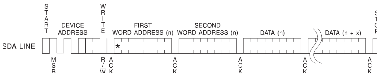
Figure 10. Page Write
