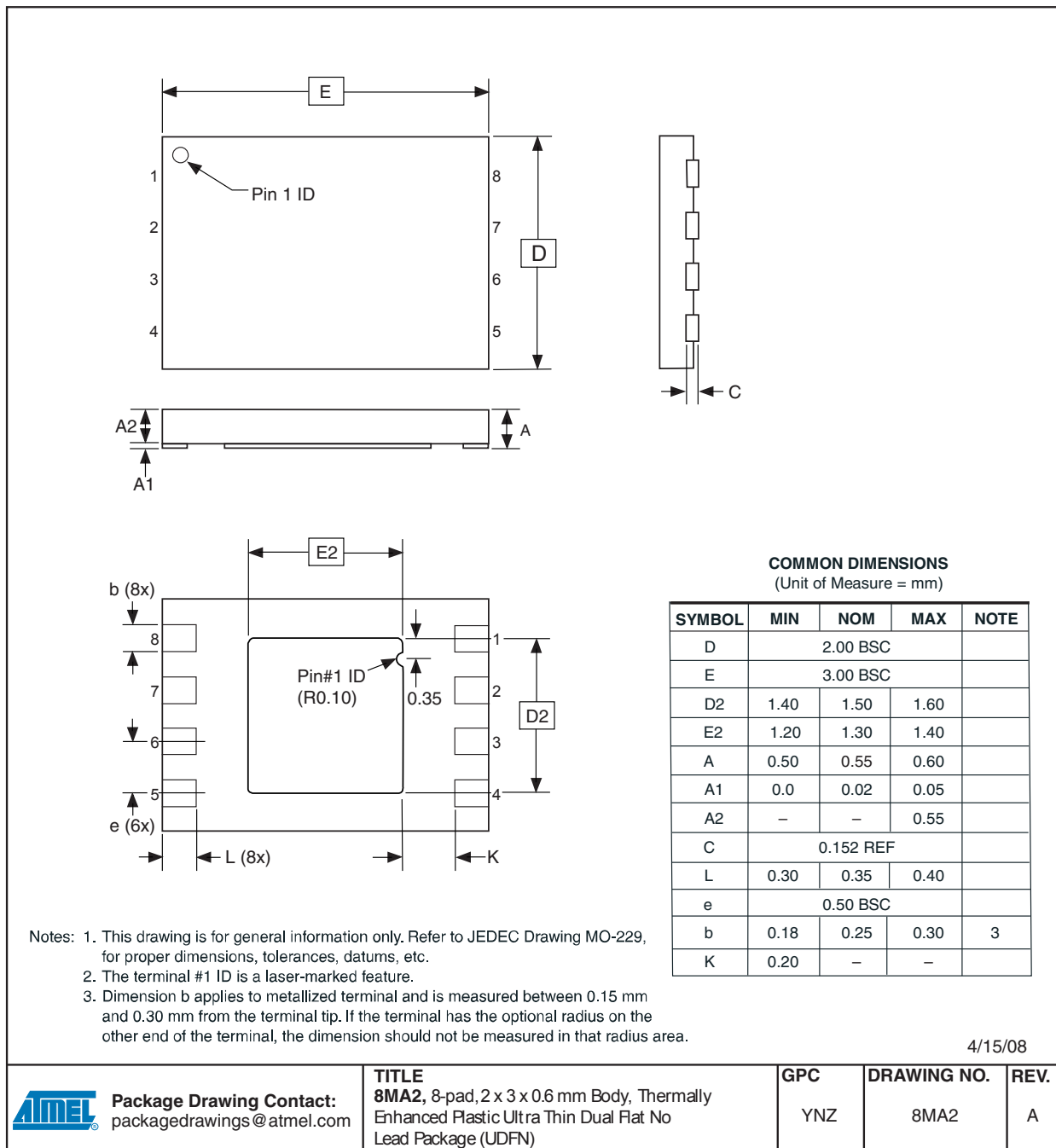
Figure 15. 8MA2 – UDFN
