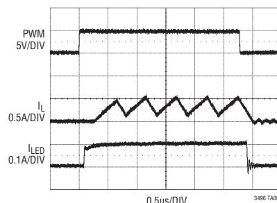
3000:1 PWM Dimming at 120Hz
