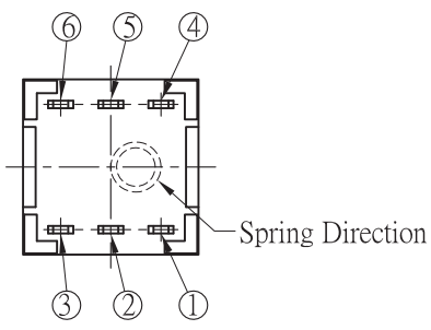
A'-A' VIEW
